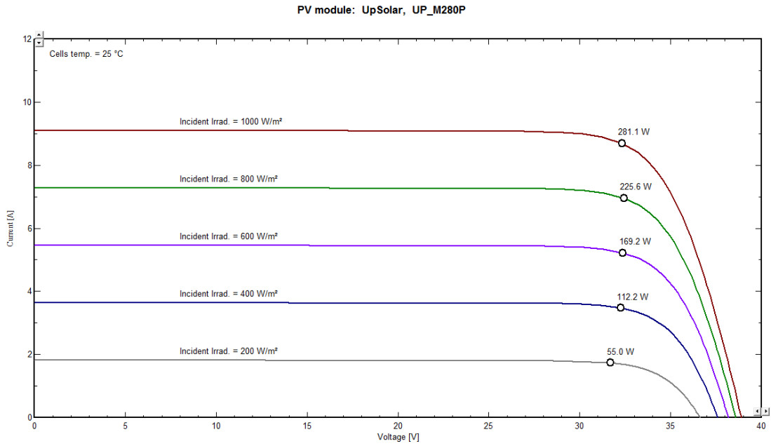
I-V curve of UP-M280P for different irradiance levels
