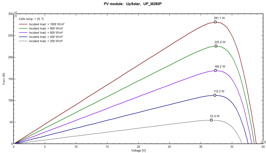
P-V curve of UP-M280P for different irradiance levels
