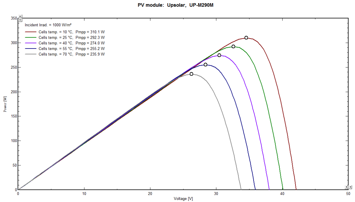
P-V curve of UP-M290M for different temperature levels
