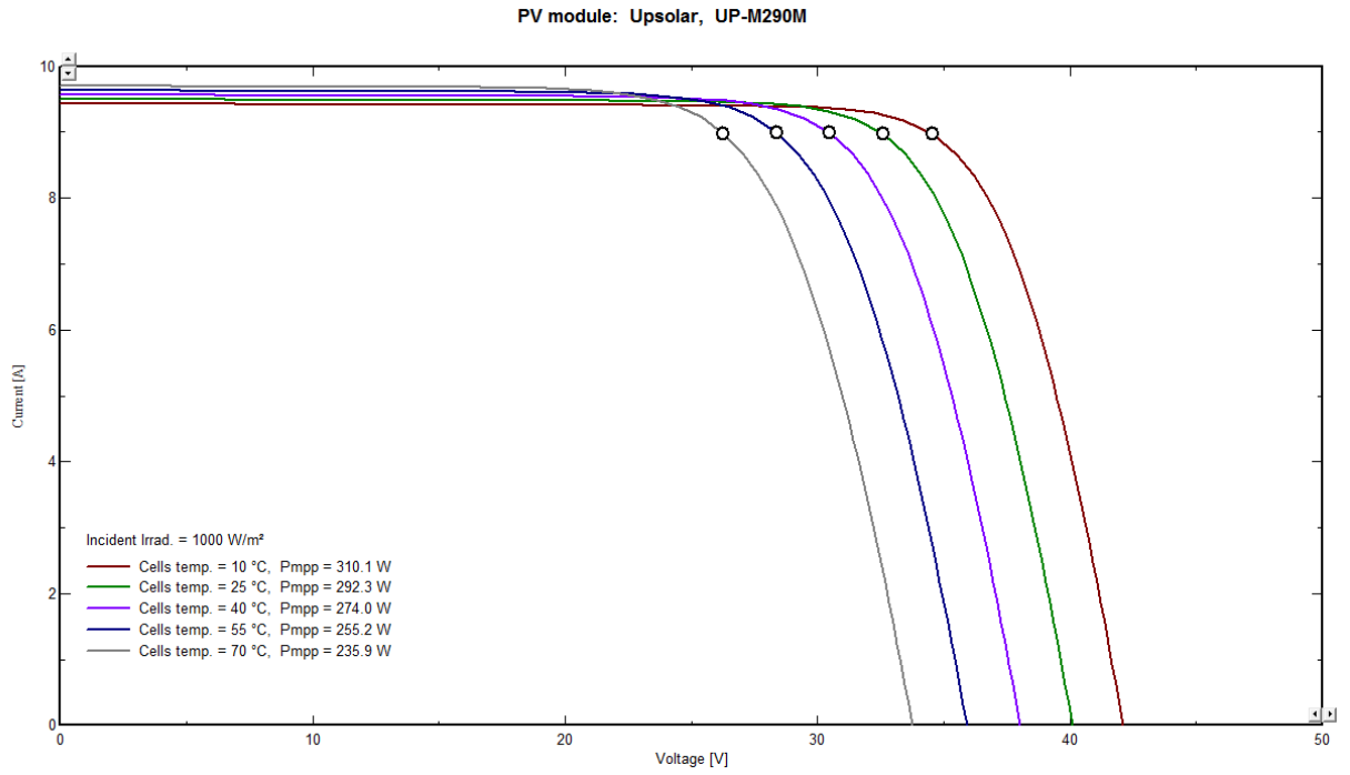
I-V curve of UP-M290M for different temperature levels
