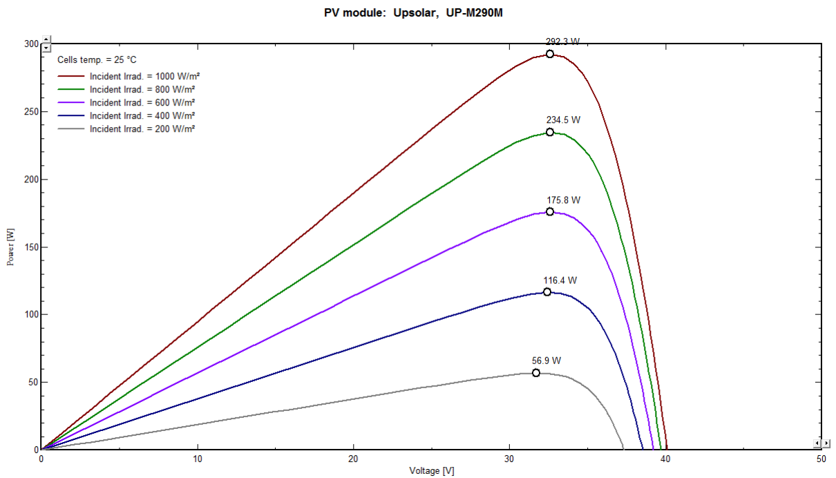
P-V curve of UP-M290M for different irradiance levels
