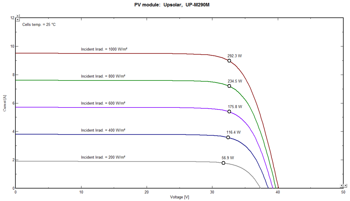
I-V curve of UP-M290M for different irradiance levels
